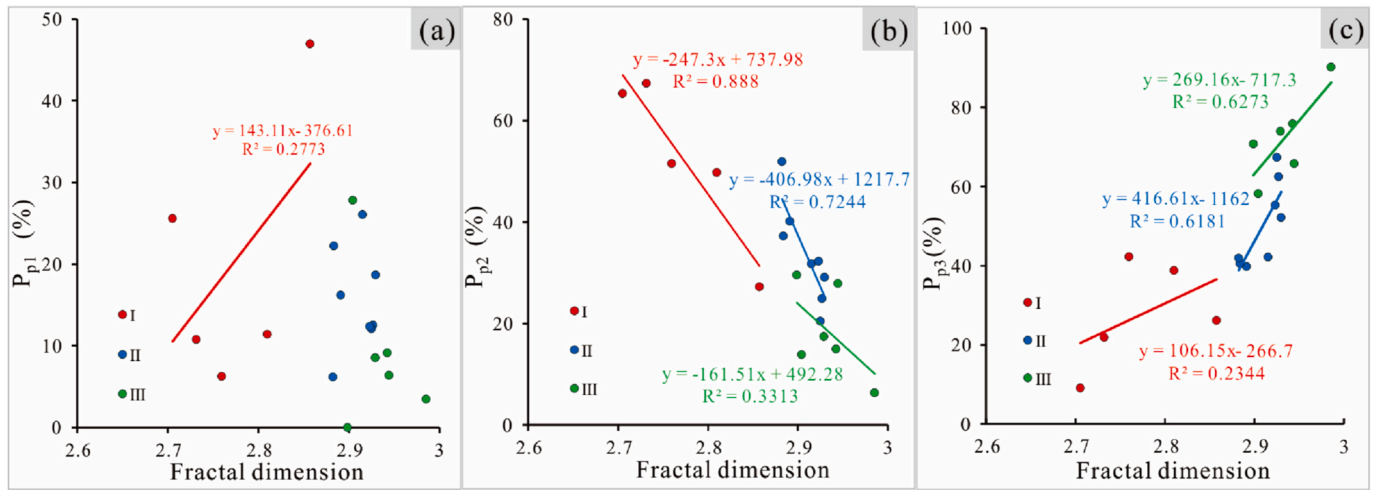
Fig. 17. The relationship between fractal dimension vs. movable fluid proportion in micron pores ( P_{p1} ) (a), submicron pores ( P_{p2} ) (b), and in nanopores ( P_{p3} ) (c).
