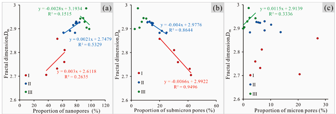
Fig. 14. The correlation of the fractal dimension with various pores. (a). Nanopores proportion, (b). Submicron pores proportion, (c). And micron pores proportion.
