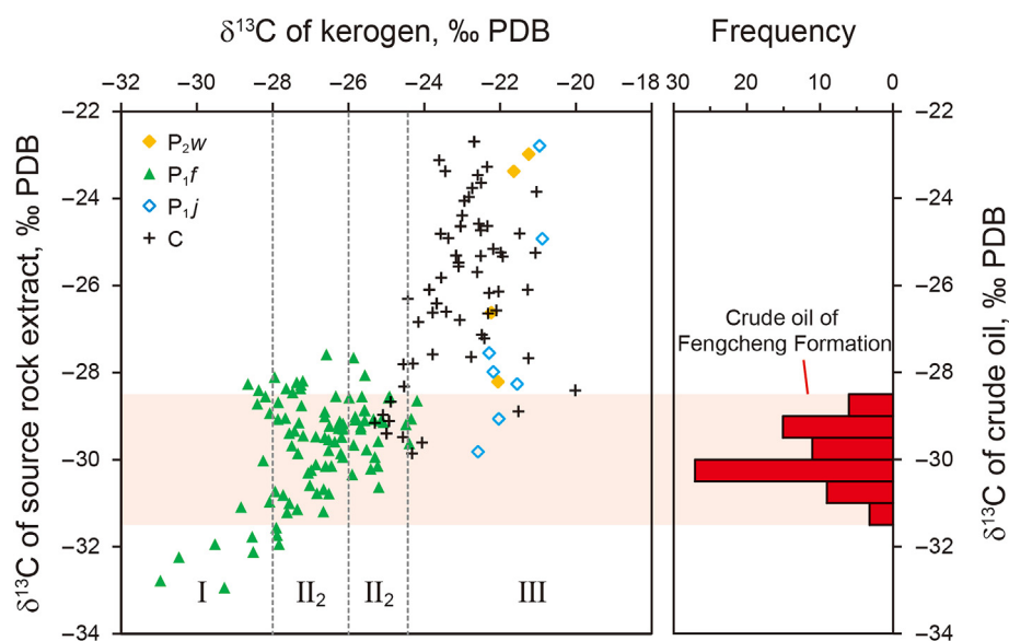
Fig. 10. Cross plot of kerogen carbon isotope and extract carbon isotope of the source rocks in different formations of Mahu Sag, and frequency distribution map of carbon isotope in the Fengcheng Formation, the Northwest Junggar Basin (modified from Dang et al., 2023).
