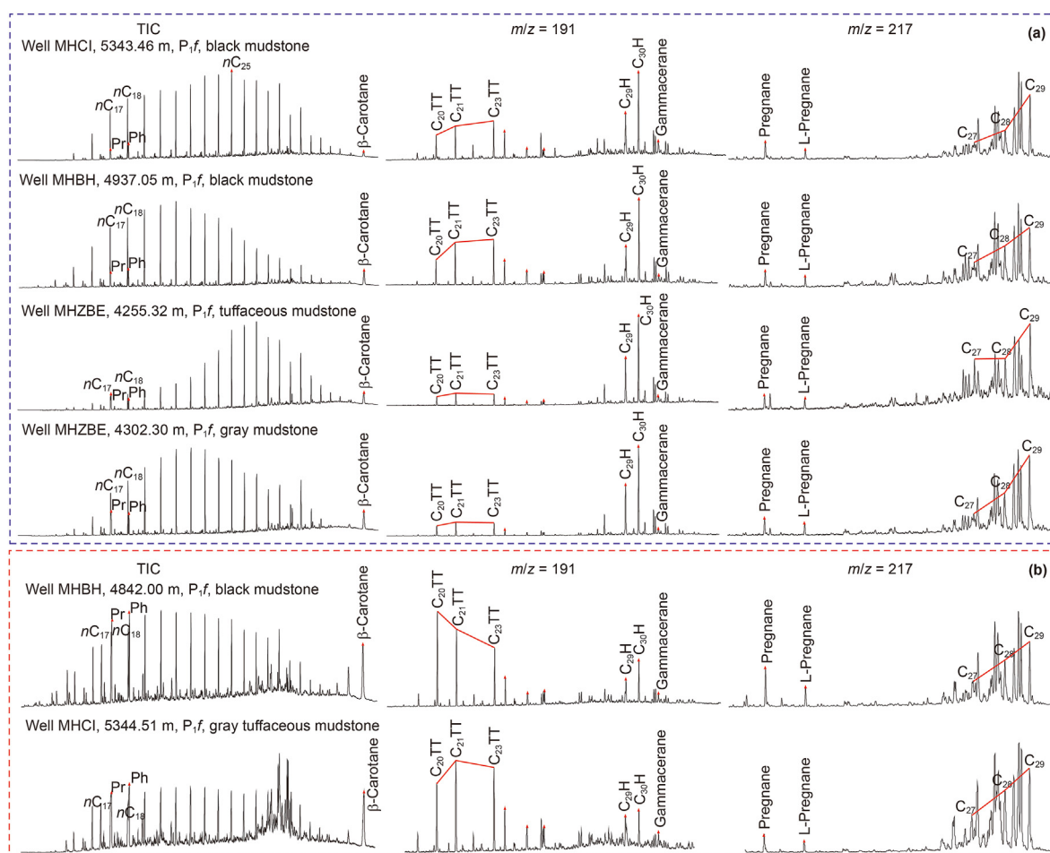
Fig. 5. Gas chromatography-mass spectrometry (GC-MS) of the saturated fraction of the Fengcheng Formation source rock samples in the southern Mahu Sag. (a) low content of tricyclic terpane and not affected by migrated hydrocarbons; (b) high content of tricyclic terpane and affected by migrated hydrocarbons.
