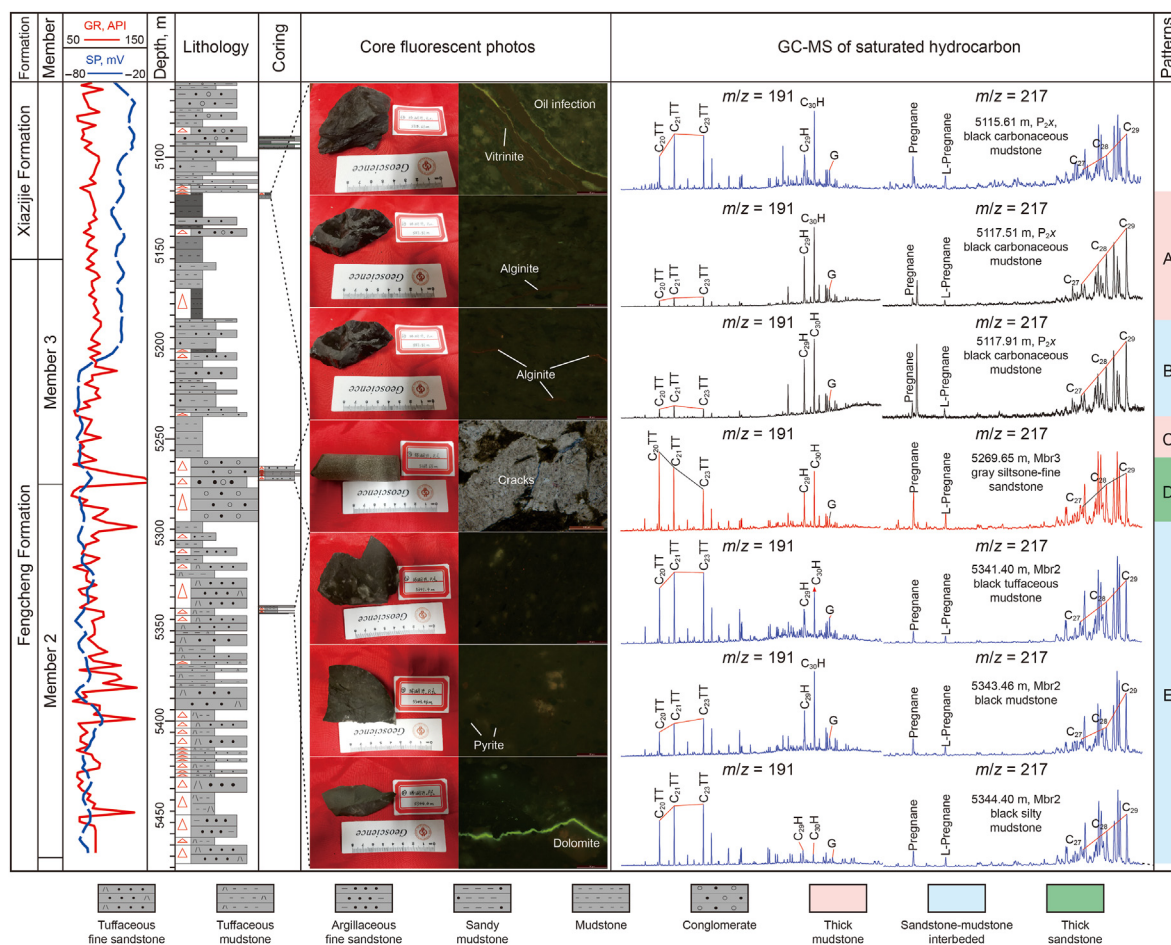
Fig. 12. Comprehensive column of lithologic assemblage and extraction GC-MS characteristics of the Fengcheng Formation in well MHCI in the south of Mahu Sag. A and C members are thick mudstones with a high maturity of extract close to sandstone and low maturity of extract far from sandstone, B and E members are sandstone-mudstone interbedded with a wide range of extract maturity, and D member is thick sandstone with high maturity of extract. (Red: crude oil biomarkers with high maturity; Blue: biomarkers of extracts from source rock affected by migrated hydrocarbons, with medium maturity; Black: biomarkers of extracts from source rock not affected by migrated hydrocarbons, low maturity.)
