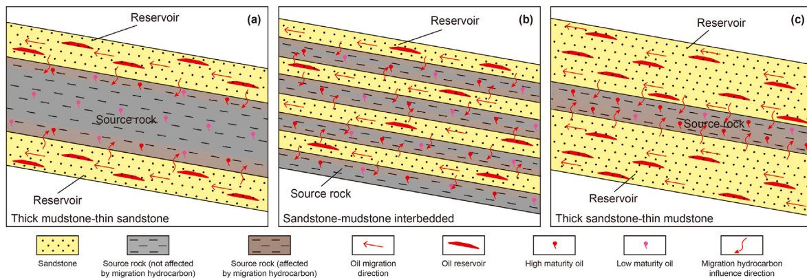
Fig. 14. Patterns of source rock affected by migrated hydrocarbons of the Fengcheng Formation in the south of Mahu Sag. (a) Thick mudstone-thin sandstone pattern; (b) sandstone-mudstone interbedded pattern; (c) thick sandstone-thin mudstone pattern. The red shadow represents the zone affected by the migrated hydrocarbons.
