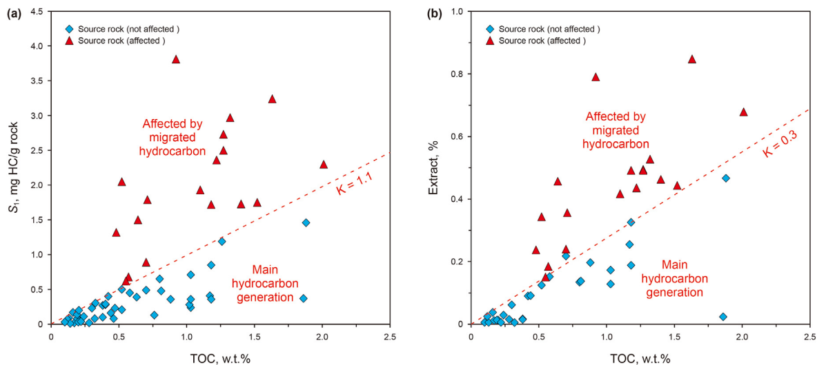
Fig. 7. Cross plots for Rock-Eval pyrolysis parameters identification of source rocks affected by migrated hydrocarbons in the Fengcheng Formation, southern Mahu Sag (Gao et al., 2017b; Li et al., 2018). (a) Rock-Eval S_1 versus TOC; (b) Extract versus TOC. The isocline of 1.1 of S_1 /TOC ratio and 0.3 of Extract/TOC ratio (red line) is the maximum relative hydrocarbon generating quantity. The source rocks affected by migrated hydrocarbons fall in the area above the isocline.
