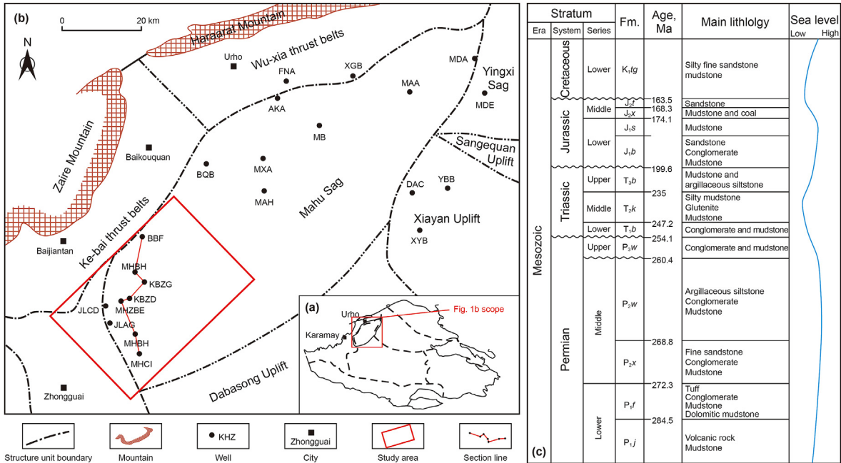
Fig. 1. (a) Location of the Mahu Sag in Junggar Basin. (b) Location of the wells and structural units of the Mahu Sag (The red polygon represents the study region). (c) Stratigraphic column of the Mahu Sag, the lithology of the Fengcheng Formation mainly includes tuffaceous sandstone, conglomerate, and mudstone (Ge, 2020). Fm. = Formation.
