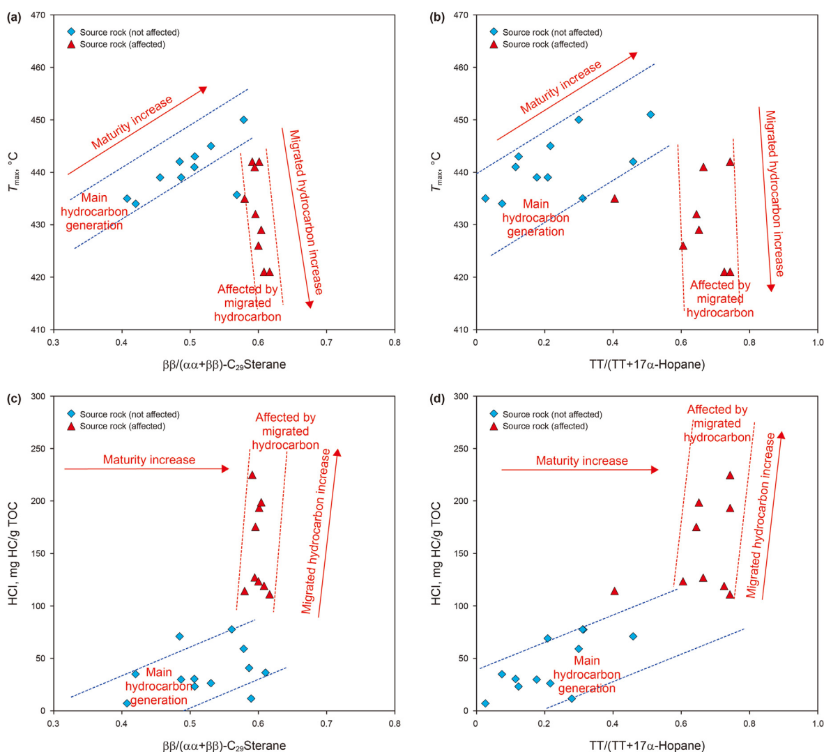
Fig. 4. Cross plots of Rock-Eval pyrolysis parameters and maturity parameters of the Fengcheng Formation source rocks affected by migrated hydrocarbons in the south of Mahu Sag. (a) T_{\max} versus \beta\beta/(\alpha\alpha+\beta\beta) -C 29 -Sterane; (b) T_{\max} versus TT/(TT+17 \alpha -Hopane); (c) HCl versus \beta\beta/(\alpha\alpha+\beta\beta) -C 29 -Sterane; (d) HCl versus TT/(TT+17 \alpha -Hopane).
