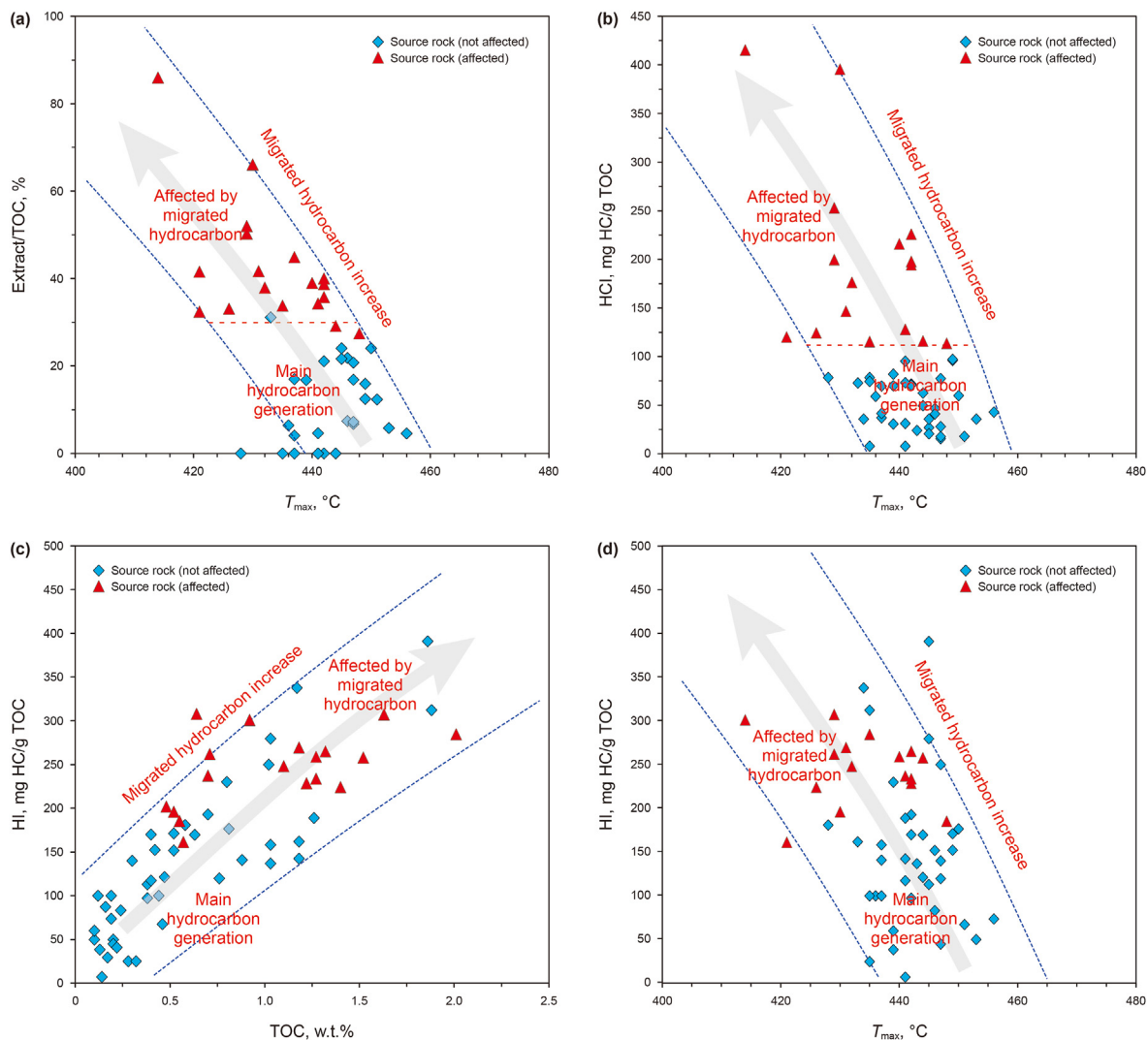
Fig. 8. Cross plots of (a) Extract/TOC versus T_{max} , (b) HCl versus T_{max} , (c) HI versus TOC, and (d) HI versus T_{max} of the Fengcheng Formation source rock samples in the south of Mahu Sag.
