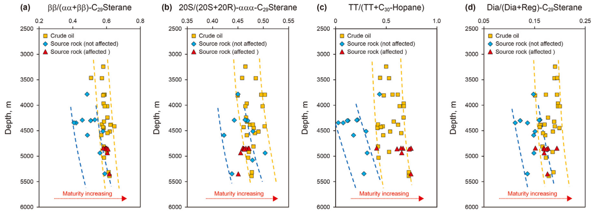
Fig. 11. Comparison plot of oil-source maturity parameters of the Fengcheng Formation in the south of Mahu Sag. (a) \beta\beta/(\alpha\alpha+\beta\beta) -C 29 -Sterane versus Depth, (b) the 20S/(20S + 20R)- \alpha\alpha -C 29 -Sterane versus Depth, (c) TT/(TT + 17 \alpha -Hopane) versus Depth, and (d) Dia/(Dia + Reg)-C 29 -Sterane versus Depth (Dia: Diasteranes, Reg: regular steranes). The maturity of crude oil is higher than that of in-situ source rock at the same depth, and the maturity of source rock affected by migrated hydrocarbons is between them.
