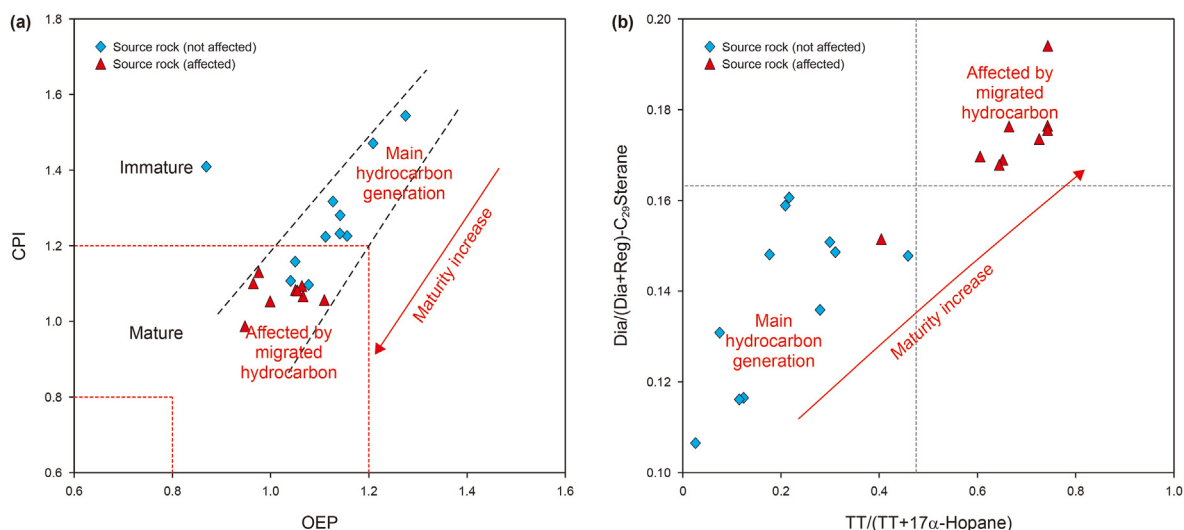
Fig. 6. Relationships between (a) OEP and CPI, (b) TT/(TT+17\alpha\text{-Hopane}) and Dia/(Dia + Reg)\text{-}C_{29}\text{-Sterane} of Fengcheng Formation source rock samples in the south of Mahu Sag.
