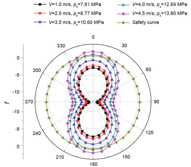
Fig. 4 Effect of the tripping in speed on wellbore stability ( a=b=10 mm)
