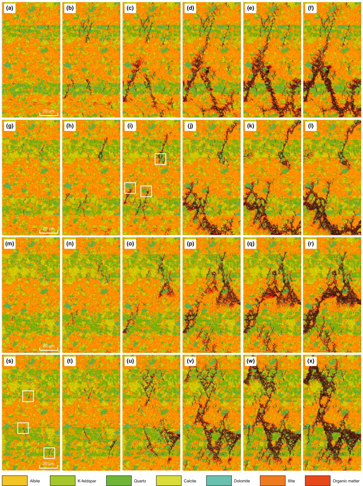
Fig. 17. Failure modes of FM-CIMs 1–4 with increasing felsic mineral lamina thickness. The white boxes highlight the initially generated microfractures. Others are the same as Fig. 15, but for FM-CIMs 1–4.
