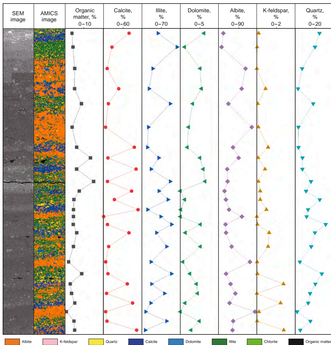
Fig. 6. Mineral content variation of different laminae in the shale sample, 3233.07 m, G108-8 well (modified from Fan, 2023).
