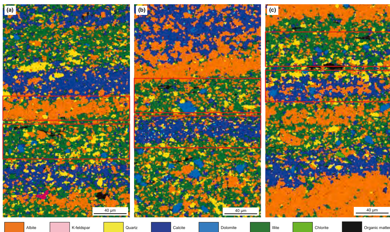
Fig. 8. Common lamina combination types of shales in the Kong-2 Member of Cangdong Sag, Bohai Bay Basin. (a) Felsic-mineral-clay-mineral laminaset, 3233.07 m, G108-8 well. (b) Carbonate-mineral-clay-mineral laminaset, 3233.07 m, G108-8 well. (c) Mixed-mineral-clay-mineral laminaset, 3233.07 m, G108-8 well (modified from Fan, 2023).
