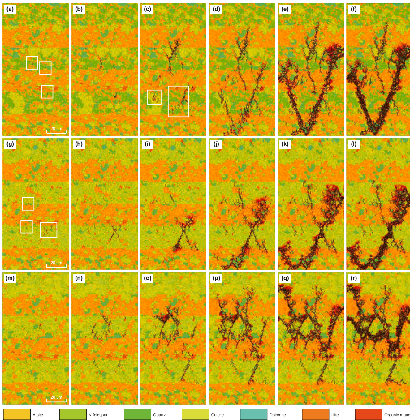
Fig. 15. Failure mode diagrams of the FM-CIMs, CaM-CIMs, and MM-CIMs. White boxes highlight the initially generated microfractures. (a) shows the failure mode of the FM-CIMs near failure, but undamaged. (b), (c), (d), and (e) manifest the failure modes of the FM-CIMs at the early, middle, and late stages of failure, and when failure is complete, respectively. (f) presents the failure mode after displacement loading. (g) reveals the failure mode of the CaM-CIMs model near failure, but undamaged. (h), (i), (j), and (k) exhibit the failure modes of the CaM-CIMs at the early, middle, and late stages of failure, and when failure is complete, respectively. (l) demonstrates the failure mode after displacement loading. (m) displays the failure mode of the MM-CIMs near failure but undamaged. (n), (o), (p), and (q) represent the failure modes of the MM-CIMs model at the early, middle, and late stages of failure, and when failure is complete, respectively. (r) shows the failure mode after displacement loading.
