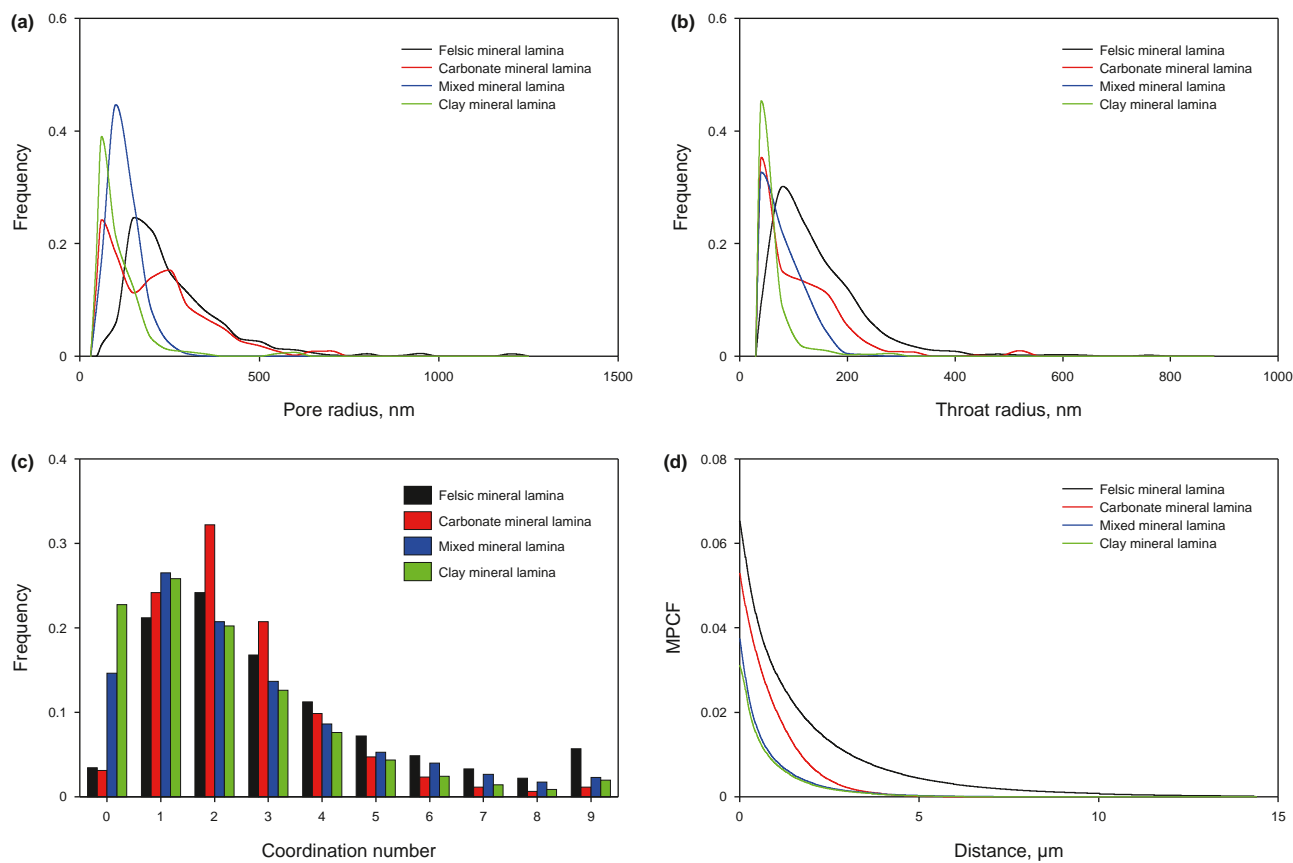
Fig. 10. Pore radius distribution, throat radius distribution, coordination number distribution, and multiple-point correlation function (MPCF) of four kinds of laminae. The MPCF indicates the pore connectivity.
