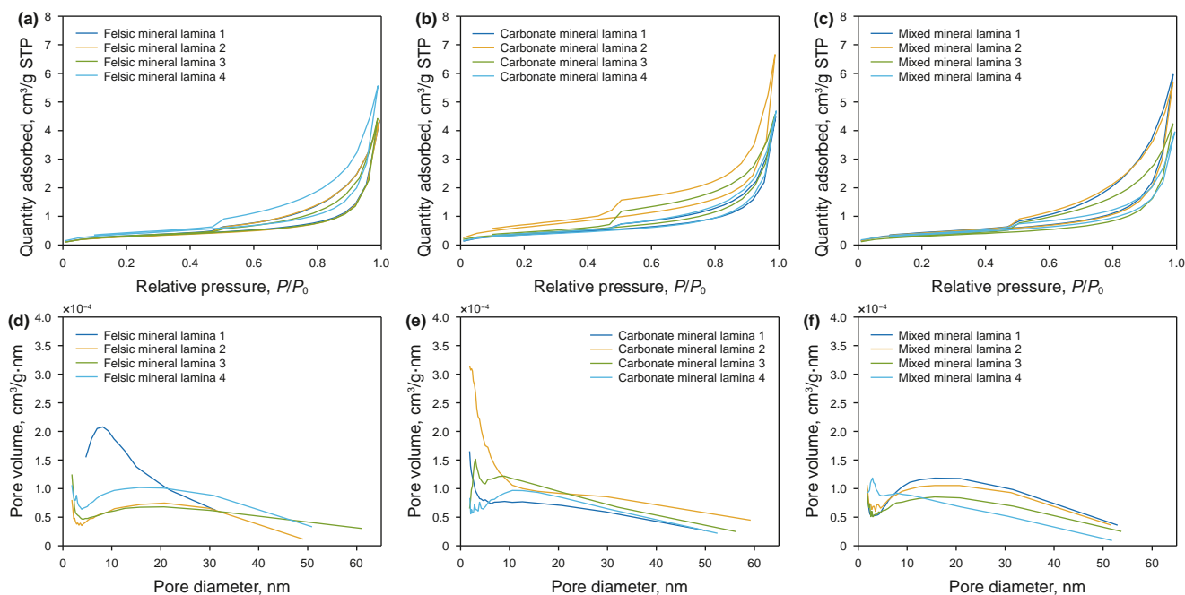
Fig. 11. The low-pressure N 2 adsorption curves and mesopore diameter distribution of four kinds of laminae. P and P_0 represent relative pressure and saturated vapor pressure, respectively. Felsic mineral lamina 1, 3852.56 m, GD12 well. Felsic mineral lamina 2, 3873.68 m, GD12 well. Felsic mineral lamina 3, 4137.78 m, GD14 well. Felsic mineral lamina 4, 4119.8 m, GD14 well. Carbonate mineral lamina 1, 3836.39 m, GD12 well. Carbonate mineral lamina 2, 3894.21 m, GD12 well. Carbonate mineral lamina 3, 4087.15 m, GD14 well. Carbonate mineral lamina 4, 4131.7 m, GD14. Mixed mineral lamina 1, 4085.95 m, GD14 well. Mixed mineral lamina 2, 4117.26 m, GD14 well. Mixed mineral lamina 3, 4127.78 m, GD14 well. Mixed mineral lamina 4, 4143.61 m, GD14 well.
