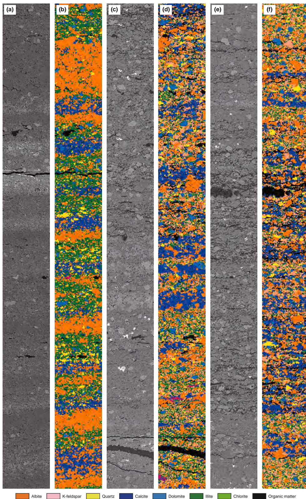
Fig. 5. Various laminae and laminasets of shales. The height and width of these images are 1.1 mm and 110 \mu\text{m} , respectively. (a)–(b) SEM and AMICS images, 3233.07 m, G108-8 well. (c)–(d) SEM and AMICS images, 3248.06 m, G108-8 well. (e)–(f) SEM and AMICS images, 3248.04 m, G108-8 well (modified from Fan, 2023).
