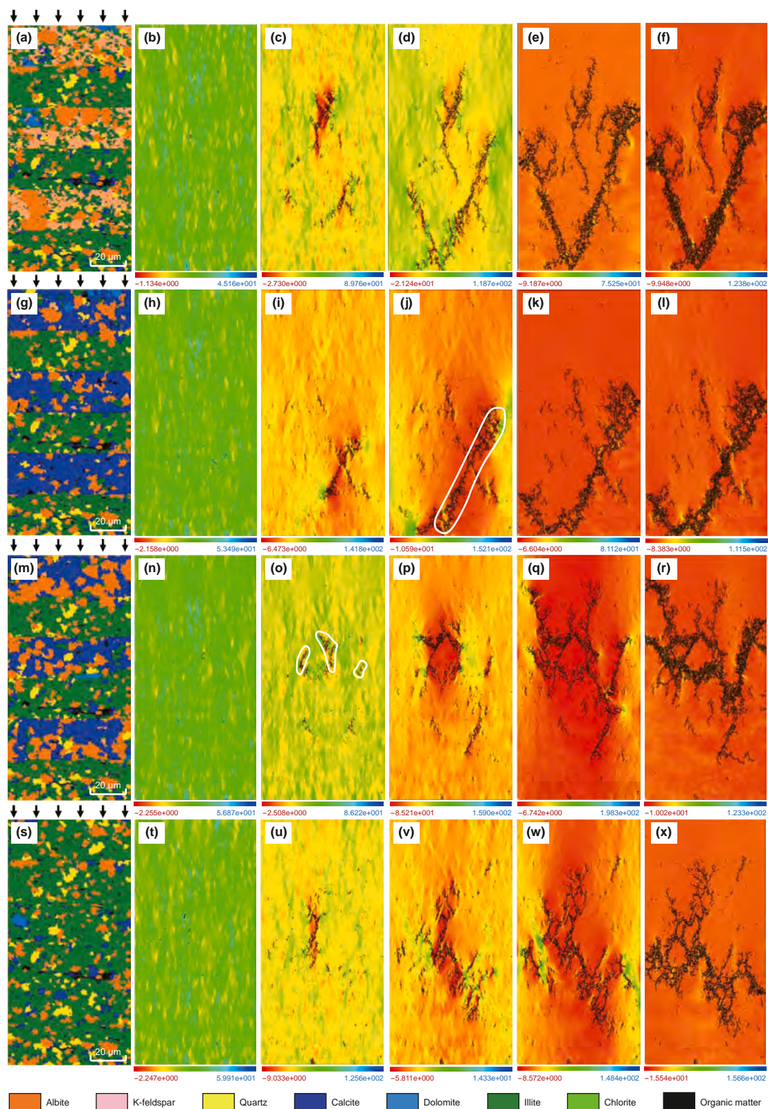
Fig. 14. Mineral compositions and maximum principal stress distribution of the felsic-mineral-clay-mineral laminaset (FM-CIMs), the carbonate-mineral-clay-mineral laminaset (CaM-CIMs), and the mixed-mineral-clay-mineral laminaset (MM-CIMs). The arrows indicate the direction of the applied force. The white ellipses highlight the key regions discussed in the text. (a), (g), and (m) represent the mineral compositions of the FM-CIMs model, CaM-CIMs model, and MM-CIMs model, respectively. (b) shows the maximum principal stress distribution of the FM-CIMs model near failure but undamaged. (c), (d) and (e) manifest the maximum principal stress distribution at the early, middle, and late stages of failure for the FM-CIMs model, respectively. (f) exhibits the maximum principal stress distribution after failure when displacement loading is applied to the FM-CIMs model for a distance. (h) shows the maximum principal stress distribution of the CaM-CIMs model near failure, but undamaged. (i), (j), and (k) demonstrate the maximum principal stress distribution at the early, middle, and late stages of failure for the CaM-CIMs model, respectively. (l) displays the maximum principal stress distribution after failure when displacement loading is applied to the CaM-CIMs model for a distance. (n) demonstrates the maximum principal stress distribution of the MM-CIMs model
