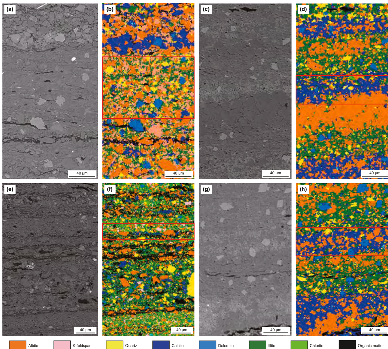
Fig. 7. Lamina types of the shales in the Second Member of Kongdian Formation of Cangdong Sag, Bohai Bay Basin, which are highlighted in the red boxes. (a)–(b) SEM and AMICS images of felsic mineral lamina, 3248.04 m, G108-8 well. (c)–(d) SEM and AMICS images of carbonate mineral lamina, 3233.07 m, G108-8 well. (e)–(f) SEM and AMICS images of clay mineral lamina, 3211.38 m, G108-8 well. (g)–(h) SEM and AMICS images of the mixed mineral lamina, 3233.07 m, G108-8 well (modified from Fan, 2023).
