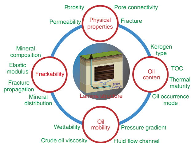
Fig. 1. Effects of lamina structure on petrophysical properties, frackability, oil mobility, and oil content of shale reservoir.
