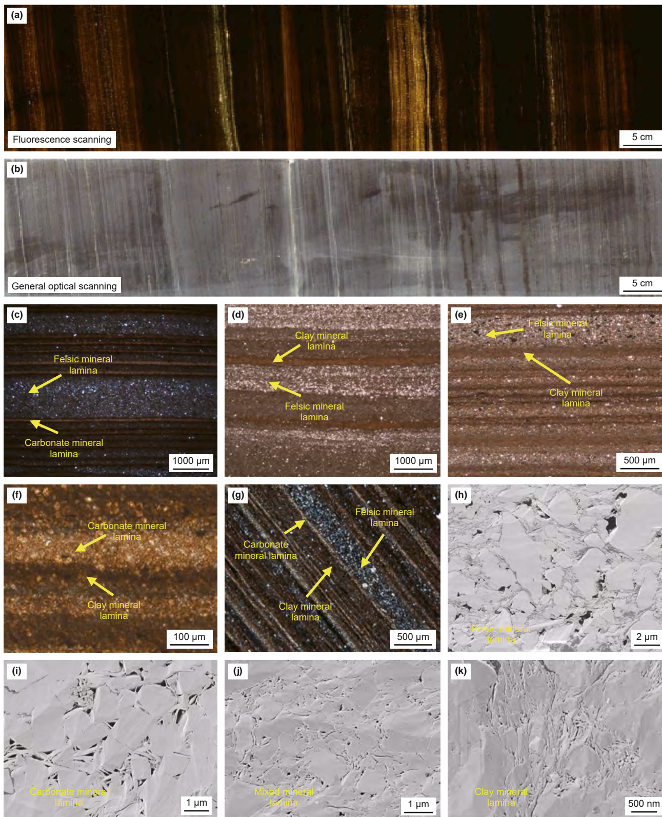
Fig. 4. Laminae and laminasets in the shales of Kongdian Formation of the Cangdong Sag in the Bohai Bay Basin, China. (a) Fluorescence scanning and (b) general optical scanning of laminated shale, 3224.5 m, G108-8 well (modified from Zhao et al., 2020a). (c) Felsic mineral and carbonate mineral laminae, 3330.66 m, G108-8 well. (d) Clay and felsic mineral laminae, 3341.65 m, G108-8 well. (e) Felsic mineral and clay mineral laminae, 2986.65 m, G108-8 well. (f) Carbonate mineral and clay mineral laminae, 3231.25.66 m, G108-8 well. (g) Felsic mineral, carbonate mineral, and clay mineral laminae, 2986.25 m, G108-8 well. (h) Felsic mineral lamina, 3280.87 m, G108-8 well. (i) Carbonate mineral lamina, 3130.97 m, G108-8 well. (j) Mixed mineral lamina, 2981.93 m, G108-8 well. (k) Clay mineral lamina, 3049.11 m, G108-8 well.
