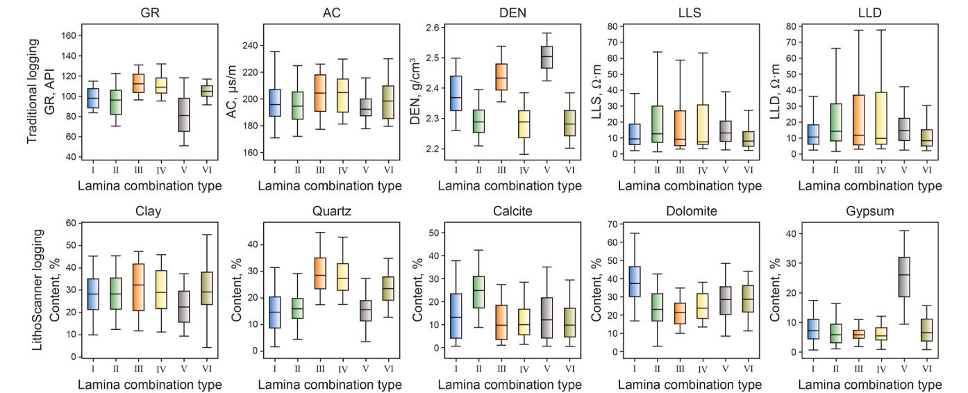
Fig. 8. Boxplots of various logging responses for different lamina combination types. I-LCC; II-BCC; III-LCF; IV-BCF; V-LCGC; VI-BCSC.
