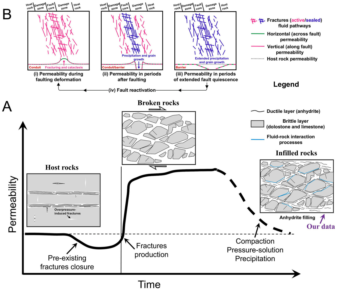
Fig. 6. (A) Schematic model illustrating the permeability evolution of the evaporite-carbonate-hosted Triassic detachment fault zone throughout a seismic cycle (modified from Uehara and Shimamoto, 2004). (B) Conceptual model showing cyclic permeability evolution of a fault zone over geological time (Pei et al., 2015).
