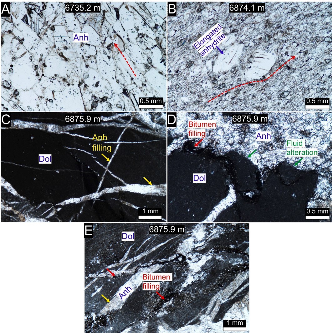
Fig. 5. Photomicrographs of thin sections from core samples obtained from borehole LS1 (see Fig. 1A), illustrating microstructural features of both intact units (A-B) and damage zone (C-E). The images highlight flow structures of anhydrite (light gray to white), along with fractures and cataclastic textures in dolostone (dark gray). Sample depths are indicated at the top center of each image. Notable features include anhydrite filling (yellow arrow), bitumen filling (red arrow), and fluid alteration (green arrow). All photomicrographs (A-E) were taken under plane-polarized light. (For interpretation of the references to colour in this figure legend, the reader is referred to the web version of this article.)
