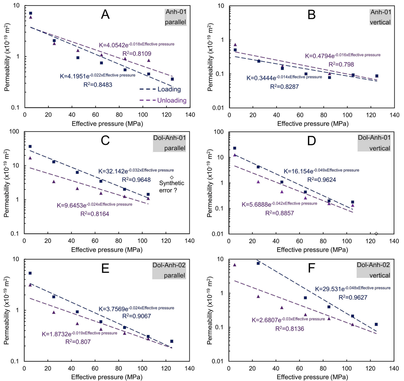
Fig. 4. Hydrostatic permeability of fault-related rocks plotted as a function of effective pressure. (A) Results for sample Anh-01 (||) from the intact unit. (B) Results for sample Anh-01 (⊥) from the intact unit. (C) Results for sample Dol-Anh-01 (||) from the damage unit. (D) Results for sample Dol-Anh-01 (⊥) from the damage unit. (E) Results for sample Dol-Anh-02 (||) from the damage unit. (F) Results for sample Dol-Anh-02 (⊥) from the damage unit. Because there are only two data points below 30 MPa, we chose to apply a global fit. Except for Anh-01(||)—where new fracture space may have formed during pressurization—the loading permeability curves for all other samples plot above their unloading curves.
