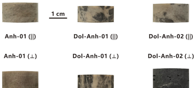
Fig. 2. Representative hand specimens of evaporite-carbonate fault rocks collected from a depth of ~6800 m. The samples include intact anhydrite (Anh-01) and mixed dolomite-anhydrite cataclasite (Dol-Anh-01 and Dol-Anh-02), each prepared with core orientations both parallel (||) and perpendicular (⊥) to the drilling direction. The samples display a heterogeneous distribution of dolomite clasts embedded within a fine-grained anhydrite matrix. The orientation definitions “||” and “⊥” also apply to Figs. 3–4 and Tables 1–2.
